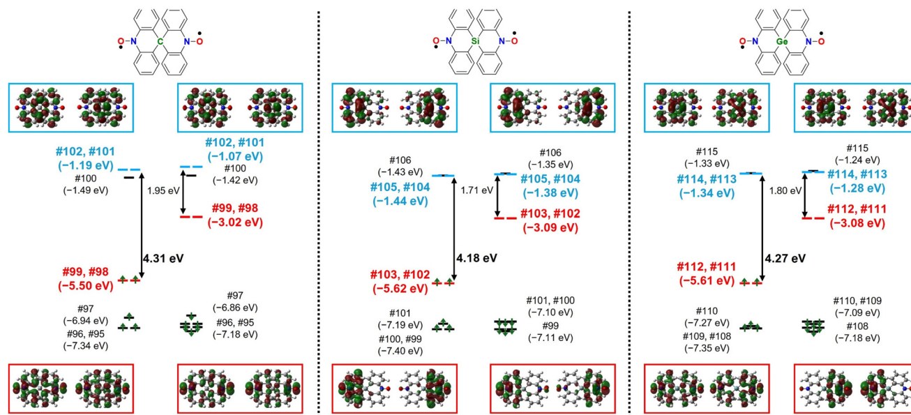
Fig. 5 Selected MO energy-level diagram for (left column) \alpha and (right column) \beta spins in the triplet state for (left) SBDO-C , (centre) -Si and (right) -Ge . The MO images are superimposed with an isovalue of 0.03. The red and blue MOs represent SOMOs and the lowest degenerate \pi^* orbital, respectively.
