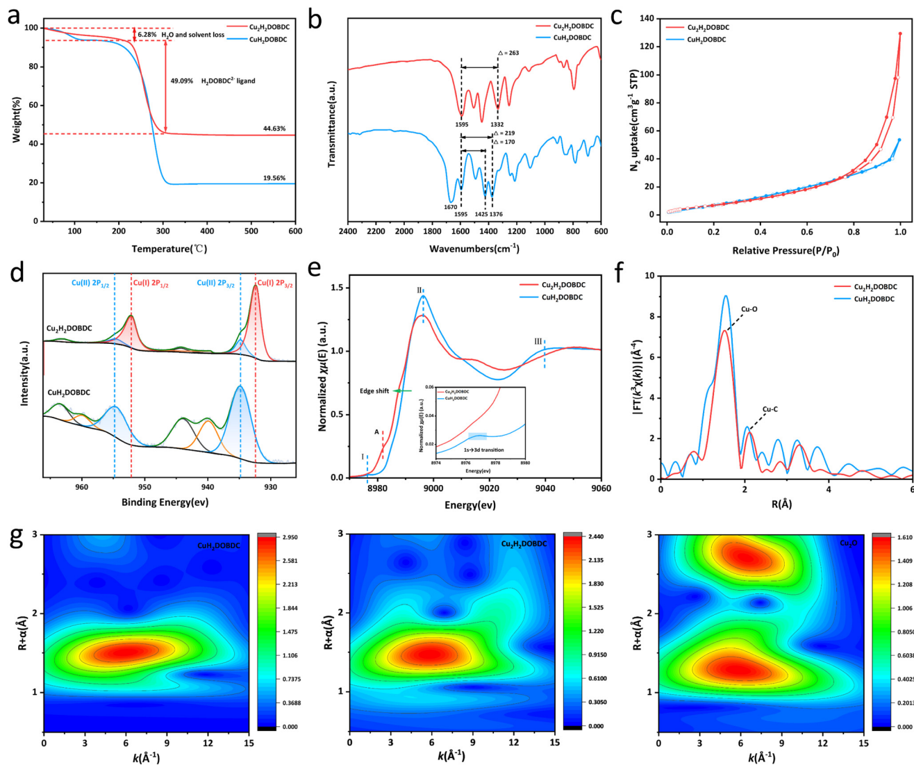
Fig. 3 (a) TGA curves for \text{Cu}_2\text{H}_2\text{DOBDC} and \text{CuH}_2\text{DOBDC} under an air atmosphere. (b) FTIR spectra of \text{Cu}_2\text{H}_2\text{DOBDC} and \text{CuH}_2\text{DOBDC} . (c) \text{N}_2 adsorption–desorption isotherms of \text{Cu}_2\text{H}_2\text{DOBDC} and \text{CuH}_2\text{DOBDC} . (d) XPS spectra for Cu 2p. (e) Cu K-edge XANES spectra. (f) Cu K-edge EXAFS spectra. (g) Wavelet transform plots the Cu K-edge EXAFS signals for \text{Cu}_2\text{H}_2\text{DOBDC} , \text{CuH}_2\text{DOBDC} and the \text{Cu}_2\text{O} standard.
