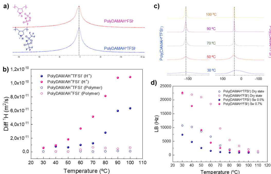
Fig. 1 ^1\text{H} SPE NMR spectra for poly(DAMAH ^+ TFSI ^- ) and poly(DAMAH ^+ FSI ^- ) at 110 °C in the dry state (a); diffusion coefficients of both protic poly(ionic liquids) by ^1\text{H} PFG NMR obtained under 75 RH% from 30 to 100 °C (b); ^{19}\text{F} SPE NMR spectra of both protic poly(ionic liquid)s under 75 RH% from 30 to 100 °C (c); and line broadening (LB) comparison between dry and swelled states (d).
