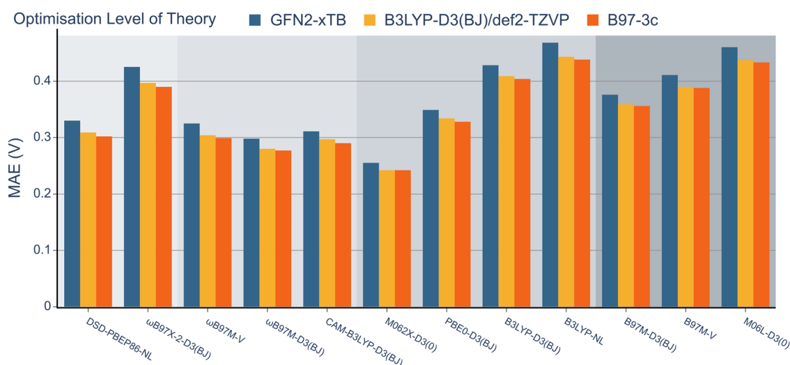
Fig. 6 MAE of redox potentials obtained with 12 different functionals with the def2-TZVP basis set. Three different DFT-based methods were used for structure generation and computation of thermodynamical corrections. They are compared for each functional. Errors are relative to the experimental OROP dataset.
