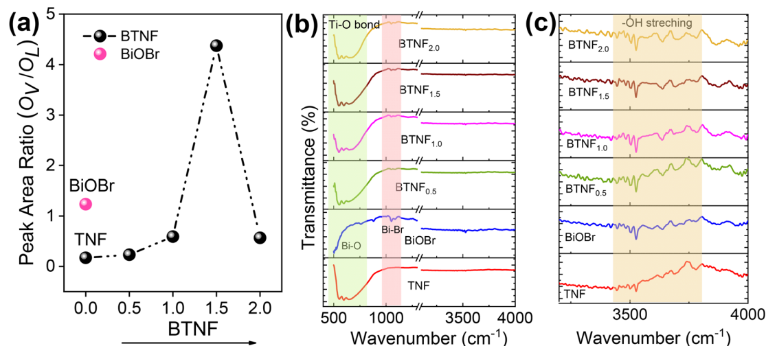
Fig. 7 (a) Peak area ratio of oxygen vacancies with lattice oxygen from XPS analysis, (b) FTIR spectrum, and (c) enlarged portion of the FTIR spectra in the 3000–4000 cm -1 range for all the photocatalysts.
