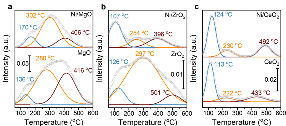
Fig. 8 \text{CO}_2 -TPD profiles at 10^\circ\text{C min}^{-1} for (a) MgO, (b) \text{ZrO}_2 , (c) \text{CeO}_2 supports, and their corresponding Ni loaded catalysts where grey dots represent the smoothed raw profiles and the solid color lines indicate the fitting results for weak, medium and strong basic sites at different temperatures.
