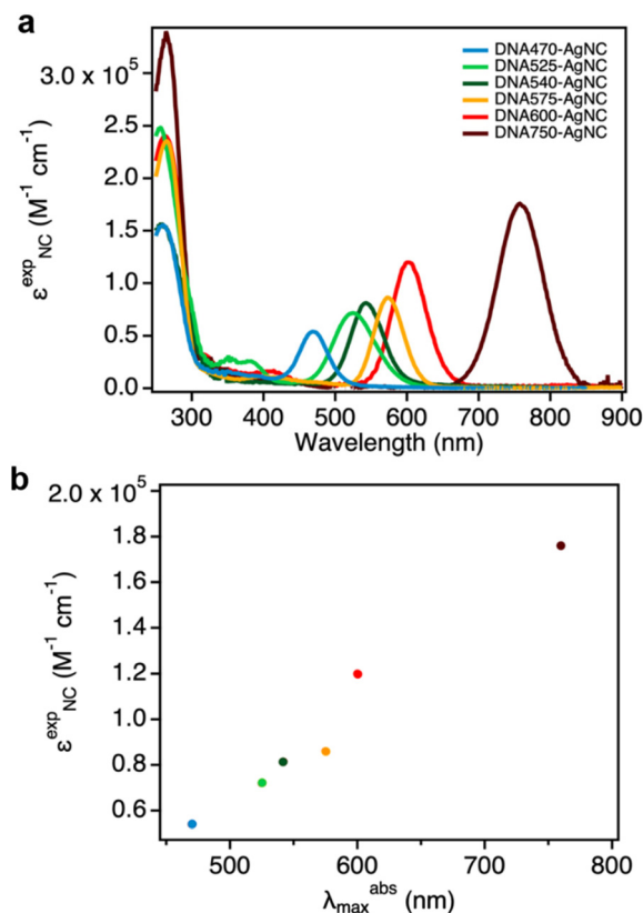
Fig. 2 (a) Normalized absorption spectra of selected DNA-AgNCs expressed in units of \epsilon \text{ (M}^{-1} \text{ cm}^{-1}\text{)} ; (b) experimentally-determined molar absorption coefficients ( \epsilon_{\text{NC}}^{\text{exp}} ) as a function of absorption maxima of the AgNC related peak in the Vis/NIR range ( \lambda_{\text{max}}^{\text{abs}} ).
