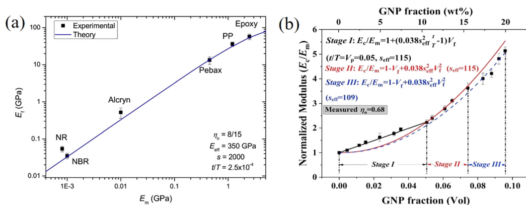
Fig. 19 (a) Variation of the modulus of grapheme nanoplatelets (GNPs) with the modulus of the matrices (dots: experiment data; blue line: theory predictions from eqn (16) and (19)). Reproduced with permission from ref. 171. Copyright 2018 Elsevier. (b) Three stages for the reinforcement of GNPs on elastomers. Reproduced with permission from ref. 153. Copyright 2019 Elsevier.
