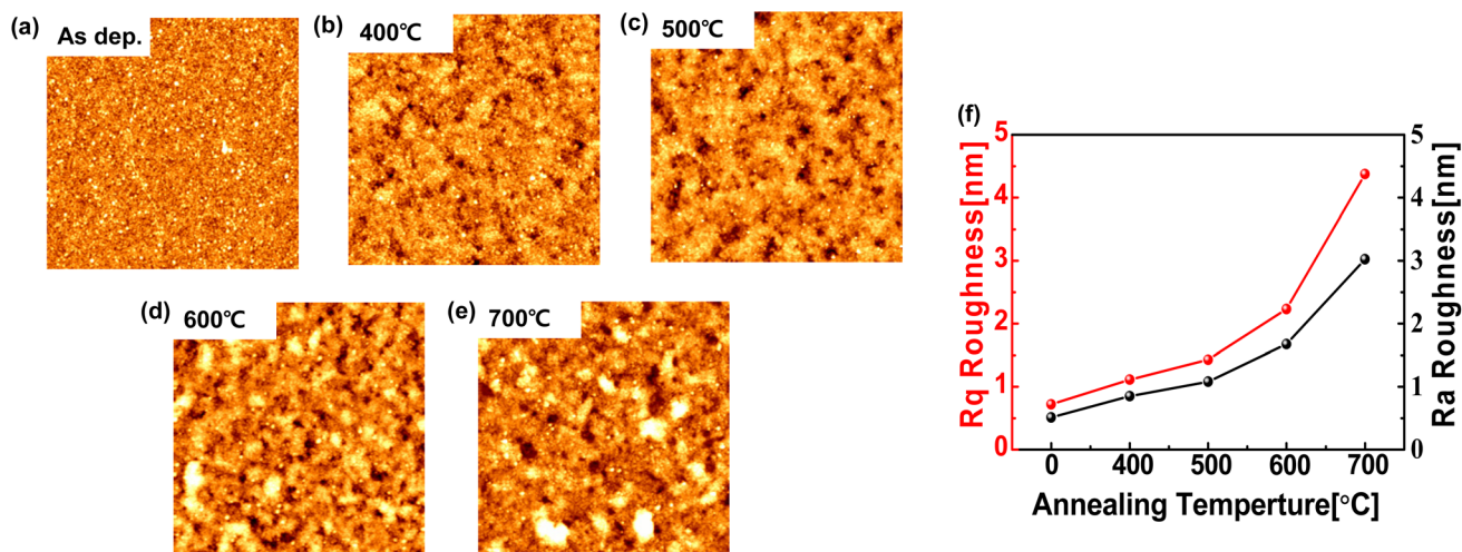
Fig. 2 AFM surface topography images of ZnO films in bilayer \text{HfO}_2/\text{ZnO} synaptic devices (a) without thermal annealing, (b) with thermal annealing at 400 °C, (c) 500 °C, (d) 600 °C, and (e) 700 °C. (f) Dependence of the root mean square ( R_q or R_{rms} ) and average roughness ( R_a ) of ZnO films on thermal annealing.
