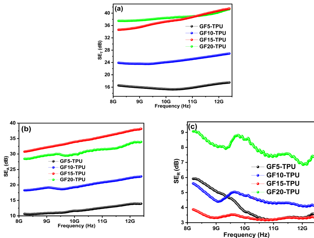
Fig. 6 EMI (a) total shielding effectiveness, SE_T , (b) shielding due to absorption, SE_A , and (c) shielding due to reflection SE_R as a function of frequency in the X-band range for the developed nanocomposites.
