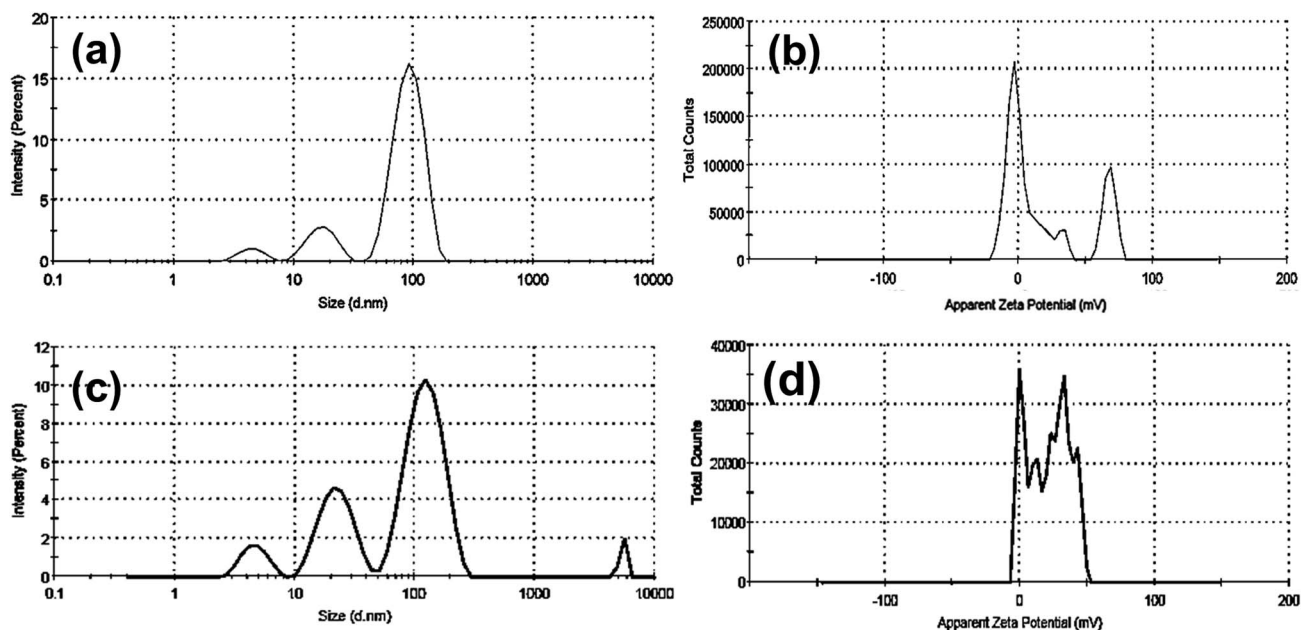
Fig. 3 DLS and zeta potential data for both CTAB- (a and b), and PVP-capped (c and d) Au-NRs.
