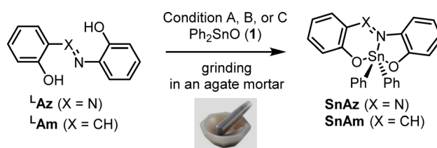
Scheme 1 Mechanochemical synthesis of \text{SnAz} and \text{SnAm} . Condition A: L/1 = 1/1 mol mol -1 , condition B: L/1 = 1/1.8 mol mol -1 , condition C: L/1 = 1/1.8 mol mol -1 with 2 drops of acetone (30 \mu\text{L} ). L: ^{\text{L}}\text{Az} or ^{\text{L}}\text{Am} .
