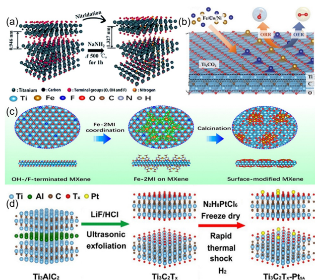
Fig. 4 (a) Synthesis procedures for the N-Ti 2 C 2 T x nanosheets and their dispersion. 46 Copyright 2018, Royal Society of Chemistry. (b) Mechanisms for the conformation of Fe/Co/Ni-DACs based on Ti 2 CO 2 and for the electrocatalytic reactions in aqueous electrolytes. 52 Copyright 2021, Wiley. (c) Schematic illustration for the preparation procedure of the surface-tuned MXene/TiFeO x nanosheets. 51 Copyright 2020, American Chemical Society. (d) Schematic illustration of constructing Pt single atoms on monolayer Ti 3 C 2 T x . 53 Copyright 2022, American Chemical Society.
