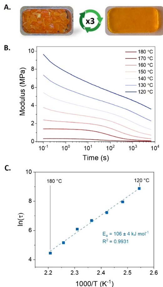
Fig. 3 (A) Thermo-mechanical recycling of photocured BEN-20 through compression molding at 150 °C under 2 tons of pressure for 30 min. (B) Stress–relaxation curves and (C) Arrhenius plots of BEN-20 after the first recycling via compression molding.
