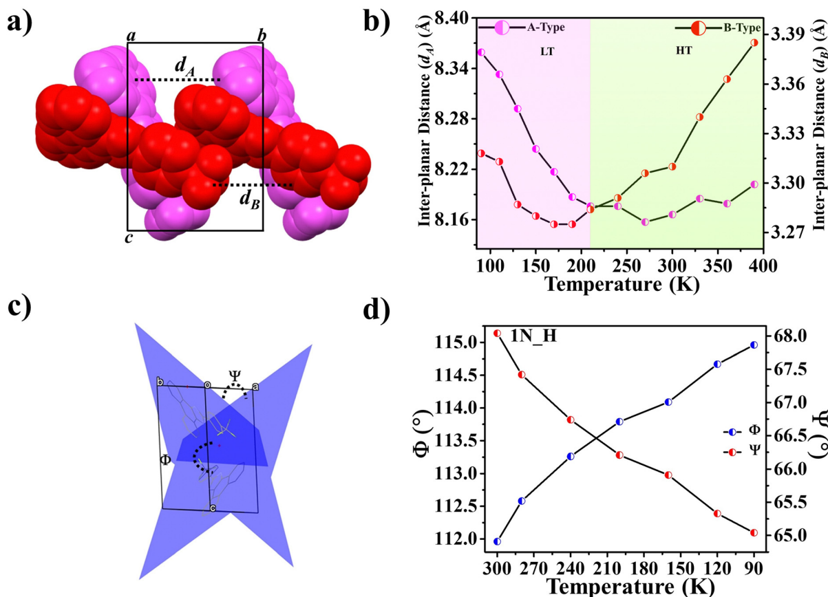
Fig. 17 For 1P_O (Fig. 4), (a) stacking of molecules A (pink) and B (red) along [010] and (b) variation of inter-planar distances d_A and d_B with temperature. For 1N_H (Fig. 4), (c) dihedral angles \Phi and \Psi between the molecular planes passing through the adjacent molecules A and B, forming an open bookcase-like geometry while viewing down [110] and (d) the variation of \Phi and \Psi with temperature. 61
