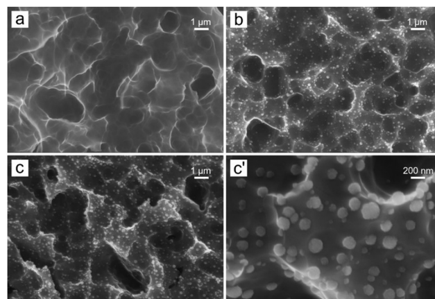
Fig. 1 SEM images of (a) untreated porous Al (sample a, no GD) and b–c–c' (porous Al samples subjected to galvanic displacement) in 0.5 mM \text{Na}_3\text{RhCl}_6 , pH 2.0, for different times: (b) t_{\text{GD}} = 1 min (sample b); (c) t_{\text{GD}} = 2 min (sample c); (c') t_{\text{GD}} = 2 min, magnified detail.
