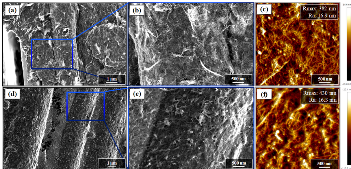
Fig. 4 SEM and AFM micrographs of the dominant p- and n-type carbon-based materials, (a)–(c): p-type material, and (d)–(f): n-type material.
