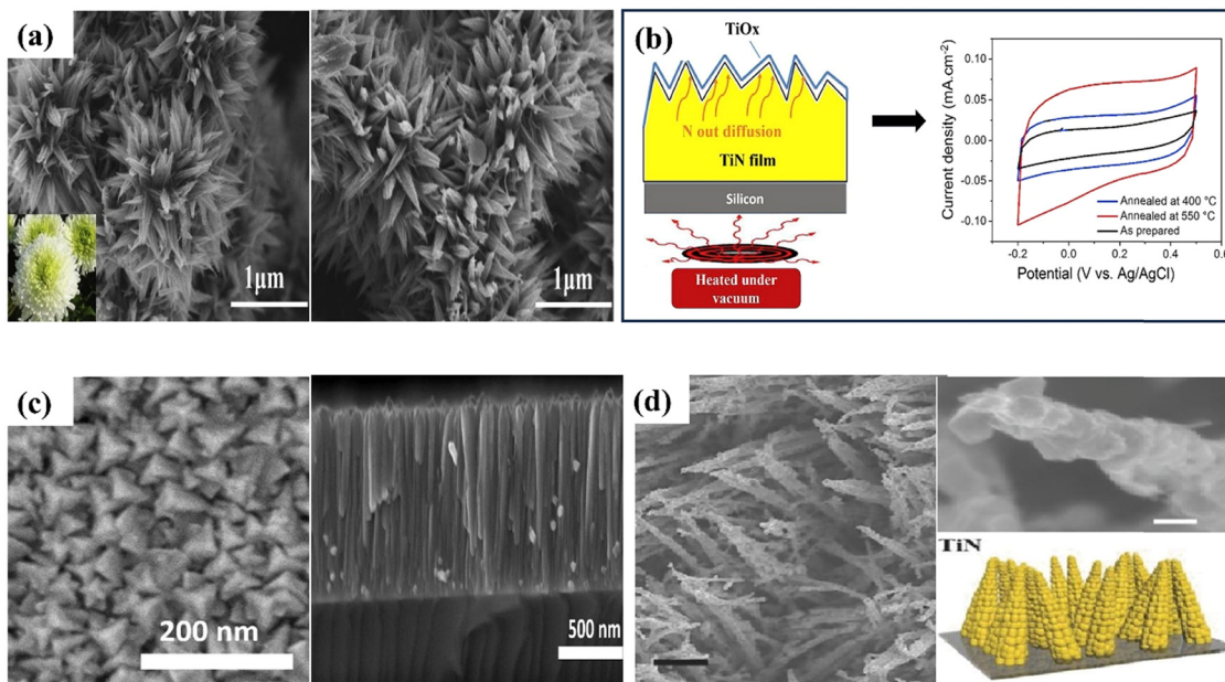
Fig. 11 SEM images of (a) CL-TiN (reproduced from ref. 152 with permission); (b) this diagram illustrates the annealing of TiN thin films in vacuum and cyclic voltammogram curves for both the pre- and post-annealing state of TiN electrodes, (c) pyramid-shaped TiN nanostructures (reproduced from ref. 155 with permission); (d) corn like TiN nanostructure (reproduced from ref. 153 with permission).
