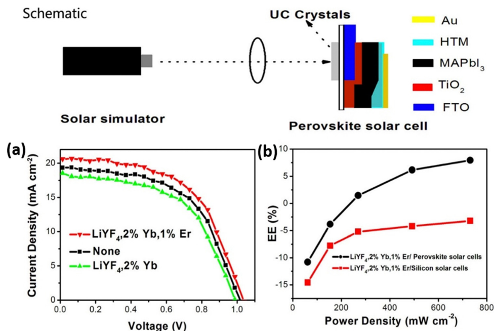
Fig. 11 A schematic representation of the perovskite solar cells under the simulated sunlight excitation. (a) J-V curves of the perovskite solar cells: LiYF 4 :2%Yb 3+ , 1%Er 3+ crystals, LiYF 4 :2%Yb 3+ crystals, and no crystals, obtained under simulated solar illumination with an intensity of 0.73 W cm -2 . (b) Enhancement efficiencies (EE) of the perovskite solar cells and silicon solar cells with LiYF 4 :2%Yb 3+ , 1%Er 3+ crystals dependent on the excitation power density. Reprinted with permission from the American Chemical Society. 66
