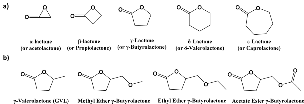
Fig. 6 (a) Types of lactones as a function of the ring size; (b) γ-valerolactone (GVL) and other examples of aprotic lactone-type solvents.
