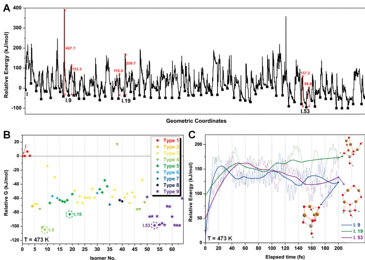
Fig. 4 (A) Computed PES along the SSW trajectory from I to I.64. (B) Relative Gibbs free energies of each isomer of I, where configurations I.9, I.19, and I.53 are marked with dashed cycles as they represent the most stable configurations of the three lower-energy isomer types (types 4, 5, and 9). (C) AIMD energies as a function of elapsed time for the evolution of I.9, I.19, and I.53 at 473 K.
