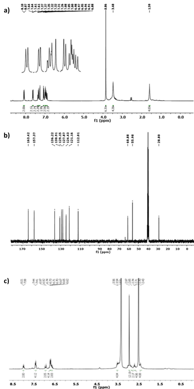
Fig. 2 The 1 H NMR (a) and 13 C NMR spectra (b) of the Schiff base ligand L 1 . (c) 1 H NMR spectrum of L 2 .
