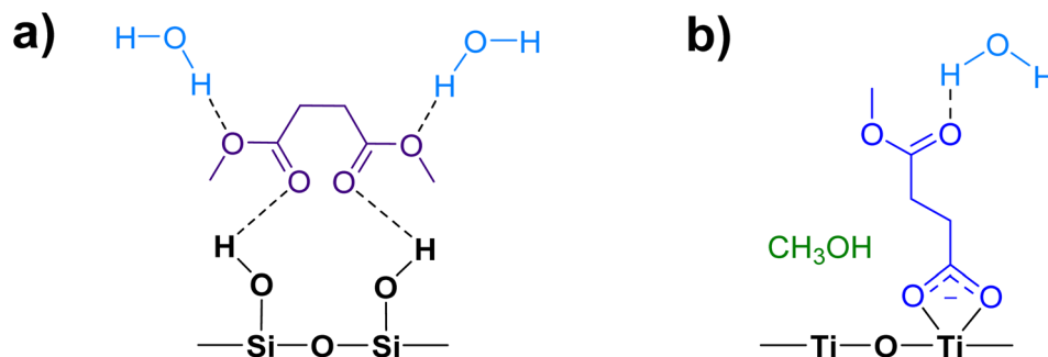
Fig. 9 Interactions of water molecules with adsorbed DMS species on (a) SiO 2 and (b) TiO 2 surfaces.
