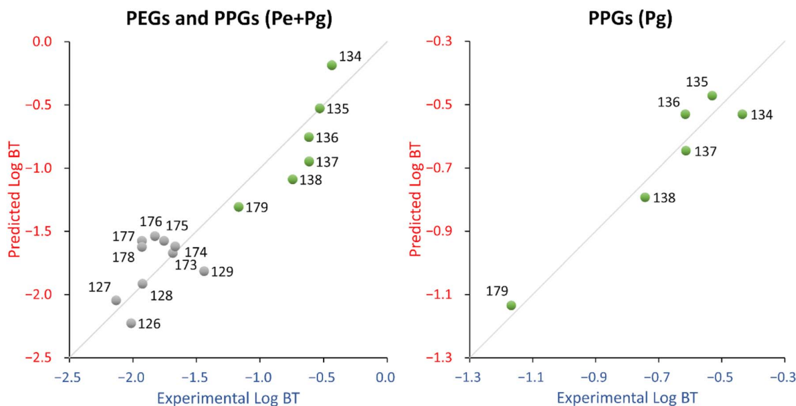
Fig. 4 Experimental vs. predicted log BT for the PEG and PPG (Pe + Pg) QSPR (left) and the PPG (Pg) QSPR (right). Gray dots = PEGs, green dots = PPGs. 126 = PEG n5, 127 = PEG n6, 128 = PEG n7, 129 = PEG n8, 134 = PPG n4, 135 = PPG n5, 136 = PPG n6, 137 = PPG n7, 138 = PPG n8, 173 = PEG n10, 174 = PEG n11, 175 = PEG n12, 176 = PEG n13, 177 = PEG n14, 178 = PEG n15, 179 = PPG n10.
