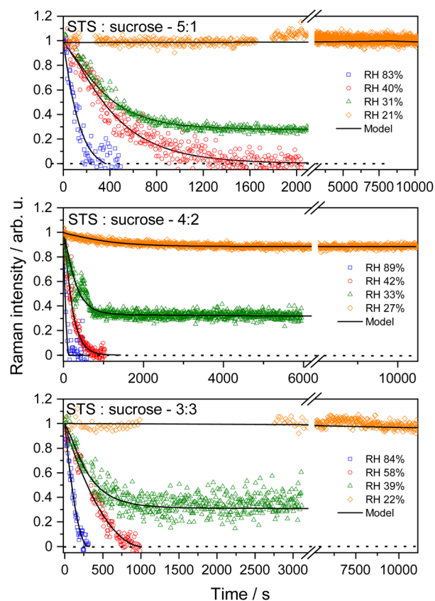
Fig. 2 Representative kinetics measurement results (symbols) of ternary STS : sucrose (5 : 1, 4 : 2 and 3 : 3 mass ratios) microdroplets exposed to ozone ( \sim 14 \text{ ppm} ) at different RHs, as well as KM-SUB model fit results (lines). The intensities shown here are the integrated Raman bands of \text{S}_2\text{O}_3^{2-}(\text{aq}) centred at \sim 445 \text{ cm}^{-1} or \sim 996 \text{ cm}^{-1} , and they are normalized to those prior to the reaction. For clarity, some apparent CERS interference is removed.
