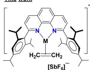
Fig. 1 Structurally characterized ethylene adducts of coinage metals supported by 1,10-phenanthroline ligands in the literature and reported in this work, [\text{L1M}(\text{C}_2\text{H}_4)][\text{SbF}_6] ( \text{M} = \text{Cu} (1), \text{Ag} (2), \text{Au} (3)) and [\text{L2Cu}(\text{C}_2\text{H}_4)][\text{BARf}] (4).
