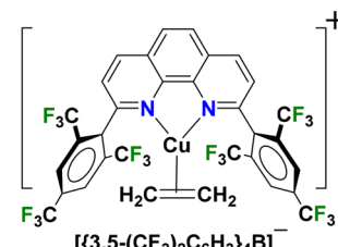
Fig. 1 Structurally characterized ethylene adducts of coinage metals supported by 1,10-phenanthroline ligands in the literature and reported in this work, [\text{L1M}(\text{C}_2\text{H}_4)][\text{SbF}_6] ( \text{M} = \text{Cu} (1), \text{Ag} (2), \text{Au} (3)) and [\text{L2Cu}(\text{C}_2\text{H}_4)][\text{BARf}] (4).
