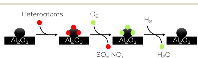
Fig. 23 Regeneration of heterogeneous Pd catalysts by oxygen from gaseous feed stream as proposed by research on sulphur Yoshimura. 137
