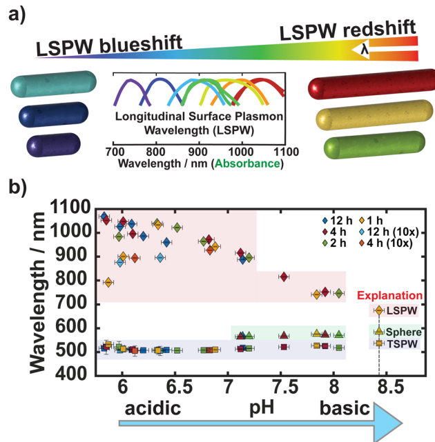
Fig. 4 (a) Scheme of correlating different GNRs lengths and their LSPW. (b) Correlation between the pH of the solutions and the LSPW ( \diamond ) and TSPW ( \square ) of the GNRs. A signature of GNSs ( \triangle ) was also observed at basic pH values. The legend states the growth times, the assignment of the absorption peaks, and the upscaling of the total solution by a factor of 10. The error bars indicate the precision of the pH measurement.
