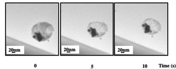
Fig. 4 "Egg" suprastructures of 4 \text{ mg mL}^{-1} of \text{Fe}_3\text{O}_4 NCs and 0.3 \text{ mg mL}^{-1} of Au NCs dispersed in an aqueous solution. The electron dose is around 1.69 \times 10^{14} \text{ e nm}^{-2} \text{ s}^{-1} .
