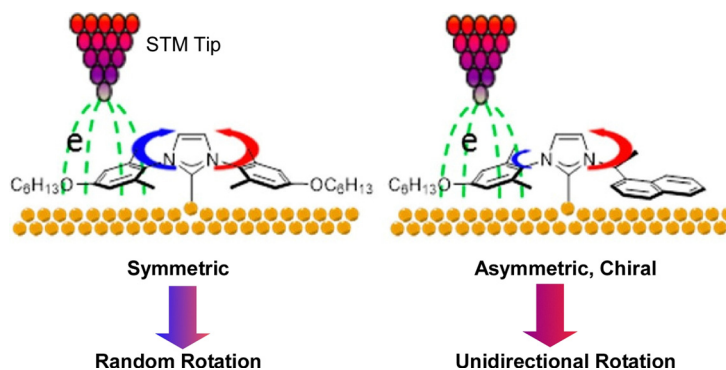
Fig. 6 Selective rotation of N-heterocyclic carbene-based surface molecular rotators driven by inelastic tunneling of electrons to the STM chip. Reprinted with permission from ref. 62. Copyright 2020 American Chemical Society.
