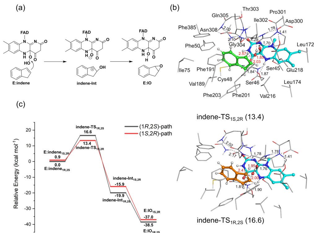
Fig. 5 (a) Mechanism of the VpInA1-catalyzed indene epoxidation and (b) the optimized structures of indene-TS 1 R ,2 S and indene-TS 1 S ,2 R . The energies, provided in parentheses in \text{kcal mol}^{-1} , are all referenced relative to E:indene 1 R ,2 S . (c) The calculated energy profiles for the VpInA1-catalyzed indene epoxidation, in which the pathways leading to the formation of (1 R ,2 S )- and (1 S ,2 R )-IO are shown in black and red, respectively. For clarity, most of the hydrogen atoms are omitted in the figure. Selected distances are given in Å.
