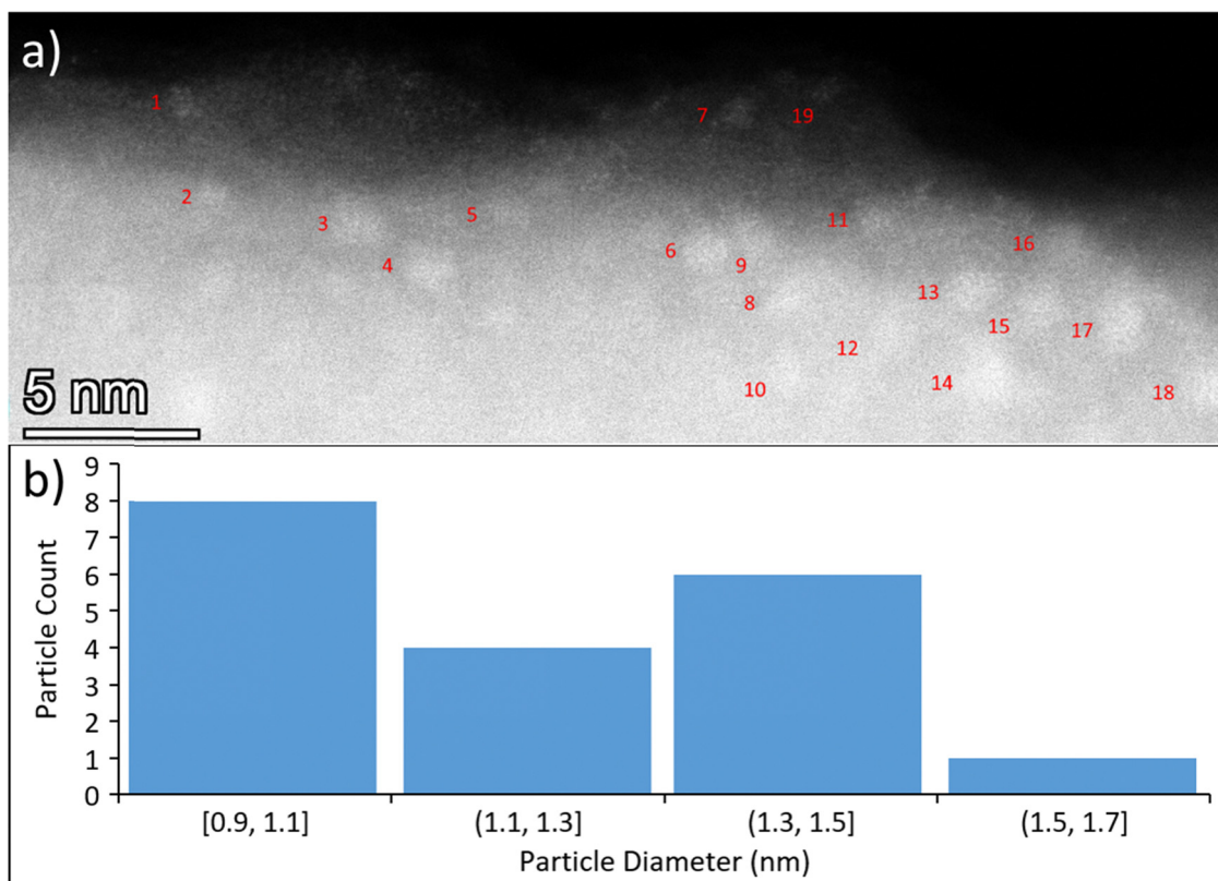
Fig. 4 STEM of CVD-Ru 3 (CO) 12 /HDS-RF-TiO 2 , showing side-on perspective of sample. (a) STEM image with numbered, encapsulated Ru clusters (cluster sizes shown individually in Table S5, ESI † ). (b) Distribution of particle diameters for encapsulated Ru clusters.
