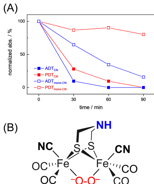
Fig. 4 (A) Comparison of the O 2 -induced decay of complexes [1–4]. At t_0 , the band intensity at 1891 cm -1 (ADT CN [1]), 1884 cm -1 (PDT CN [2]), and 1975 cm -1 (ADT mono-CN [3] and PDT mono-CN [4]) was normalized to 1 and plotted against time (spectral traces in Fig. 3 and Fig. S5, ESI†). The graph illustrates how the adt-type complexes decay faster than the pdt-type complexes, and how di-cyanide complexes decay faster than mono-cyanide complexes. (B) Most probable structure of a di-ferrous peroxide dianion intermediate of ADT CN according to DFT calculations.
