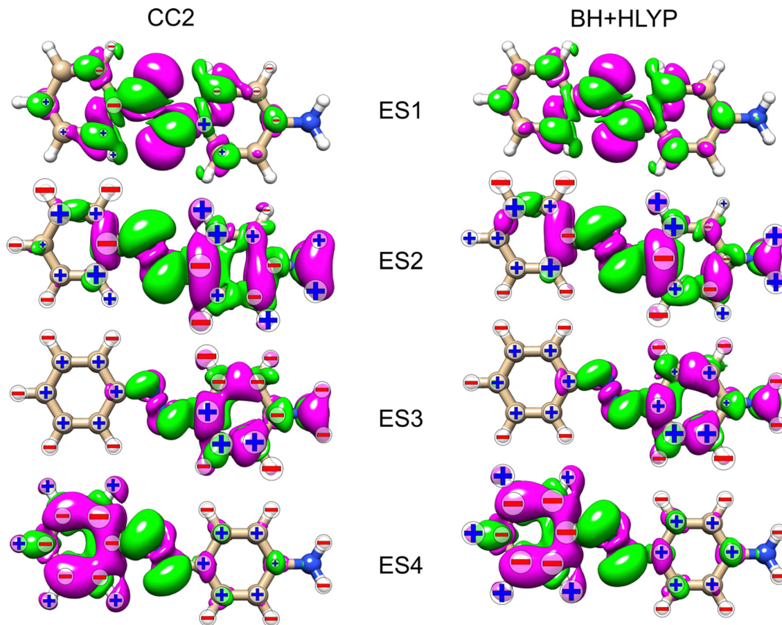
Fig. 9 AZO-2. RI-CC2 and TD-DFT/BH+HLYP (aug-cc-pwCVDZ basis set) difference densities for the four lowest excited states (ES) with the sign (+/−) of the nuclei's \mathcal{L}_K \mathcal{B}_K terms. The size of the sign indicates the magnitude (magnified by 1000) of the signal (smallest for 1 < |\text{NSCD}| < 10 , middle size for 10 < |\text{NSCD}| < 100 and largest for |\text{NSCD}| > 100 . NSCD signals with absolute values < 1 are not shown).
