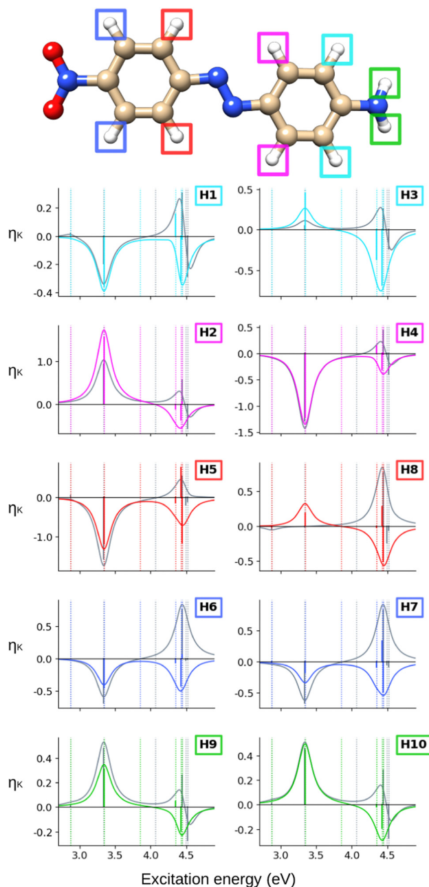
Fig. 11 AZO-3. NSCD spectra of the hydrogen nuclei. RI-CC2 (colored) and TD-DFT/BH+HLYP (grey) results with aug-cc-pwCVDZ basis set. Vertical dotted lines mark the excitation energies of the excited states. TD-DFT energies have been shifted by -0.090 eV to align the first transition with RI-CC2. The sticks have been scaled for visibility.
