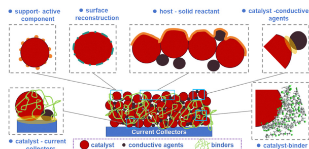
Scheme 1 A schematic depiction of the various solid–solid interfaces existing in a porous electrode.
