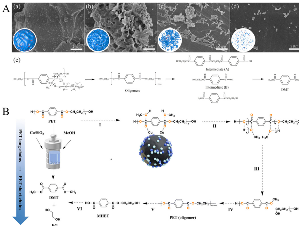
Fig. 10 (A) SEM images of remained PET at different reaction times ((a): 0 h, (b): 0.5, (c): 2 h, and (d): 4 h). (e) Possible reaction routine for the alcoholysis of PET with methanol over Ti_{0.5}Si_{0.5}O_2 . Reproduced from ref. 119 with permission from Royal Society of Chemistry, copyright [2023]. (B) Proposed reaction mechanism for PET methanolysis over the Cu/SiO_2 catalyst. Reproduced from ref. 120 with permission from Royal Society of Chemistry, copyright [2024].
