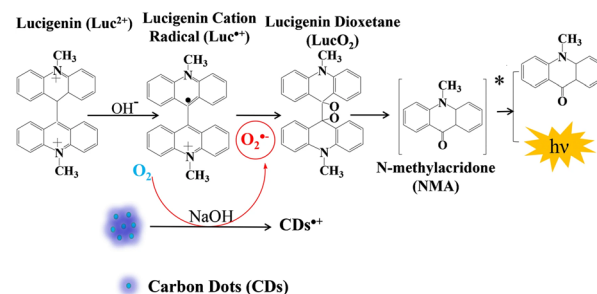
Scheme 2 Schematic representation of the lucigenin-CD system in NaOH solution. Reprinted with permission from ref. 52, Copyright 2019 Springer Nature.
