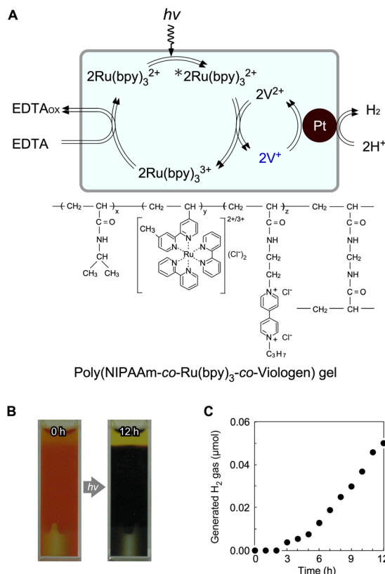
Fig. 8 (A) Photoinduced H 2 -generating system composed of a poly(NIPAAm-co-Ru(bpy) 3 -co-viologen) gel containing Pt NPs. (B) Images of the gel suspension before and after light irradiation. (C) H 2 -generation in the gel system. Reproduced from ref. 68 with permission from the Royal Society of Chemistry, Copyright 2009.
