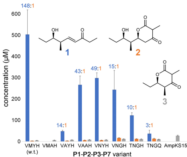
Fig. 3 Titers of 1–3 produced by P1–P2–P3–P7 and variants. Titers of 1 were quantified from peak areas of LC/MS extracted ion chromatograms using a standard curve, while 2 and 3 were quantified by UV absorption. The 1:2 ratio is indicated for each tetraketide-producing variant.
