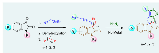
Scheme 1 Synthesis of 1,2,3-triazole fused spirooxindoles.
