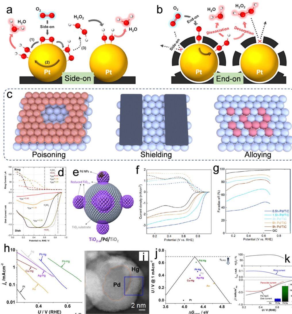
Fig. 4 \text{O}_2 adsorption on Pt/C and C(Pt)/C in the form of (a) side-on configuration and (b) end-on configuration. Reproduced from ref. 58. Copyright (2014) American Chemical Society. (c) Illustration of surface poisoning and shielding on the surface of the metal and metallic alloying. (d) Polarization curves obtained from RRDE experiments for the ORR on a Pt (111)- \text{CN}_{\text{ad}} electrode with varying \text{CN}_{\text{ad}} coverages, conducted in a 0.05 M \text{H}_2\text{SO}_4 solution. Reproduced from ref. 59. Copyright (2015) Elsevier. (e) Illustrative schematic demonstrating the encapsulation process of a \text{TiO}_{2-x} overlayer on Pd NPs via ball milling. (f) LSV curves obtained using an RRDE and corresponding (g) Faradaic efficiency for the production of \text{H}_2\text{O}_2 . Reproduced from ref. 64. Copyright (2022) American Chemical Society. (h) Kinetic current density for \text{H}_2\text{O}_2 as a function of the applied potential. (i) TEM images of the prepared Pd-Hg alloy. (j) The potential needed to achieve a kinetic current density of 1 \text{ mA cm}^{-2} for \text{H}_2\text{O}_2 on polycrystalline catalysts as a function of the calculated ^*\text{OOH} binding energy. (k) LSV curves obtained using an RRDE and corresponding \text{H}_2\text{O}_2 selectivity. Reproduced from ref. 68. Copyright (2014) American Chemical Society.
