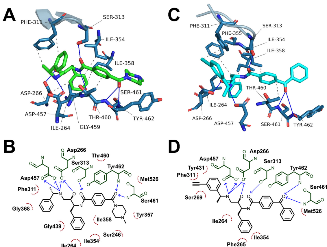
Fig. 5 (A) and (C) Interaction analyses of end-state binding modes of 49c (A, green sticks) and 20c (C, cyan sticks) in PMX. Binding site residues are shown as blue sticks, the flap region is shown as a blue cartoon representation, hydrogen bonds are shown as blue lines, hydrophobic interactions are shown as dotted grey lines. Interactions were detected using the protein ligand interaction profiler tool. (B) and (D) 2D representations of non-covalent interactions between 49c (A) and 20c (C) with binding site residues. Binding site residues are shown in green, hydrophobic interacting residues are depicted by red, dotted arcs, hydrogen bond donors are depicted as blue arrows pointing from donor to acceptor.
