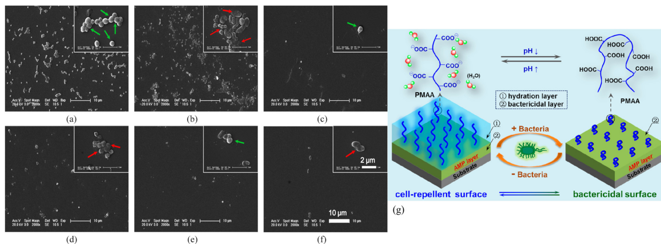
Fig. 5 S. Aureus attachment (106 cells per ml for 24 h) for (a) unmodified Si (b) AMP-grafted Si (c) one-layer PMAA (d) AMP-grafted one-layer P(VDMA-co-MAA) (e) AMP-grafted hierarchical P(VDMA- b -PHEMA) (f) AMP-grafted hierarchical P(VDMA- b -PMAA). Red arrows indicate damaged bacteria cells. (g) Schematic representation of the reversible nature of the coating. Reprinted with permission of S. Yan, et al., Nonleaching Bacteria-Responsive Antibacterial Surface Based on a Unique Hierarchical Architecture, ACS Appl. Mater. Interfaces , 2016, 8(37), 24471–24481, https://doi.org/10.1021/acsami.6b08436 . Copyright © 2016, American Chemical Society.
