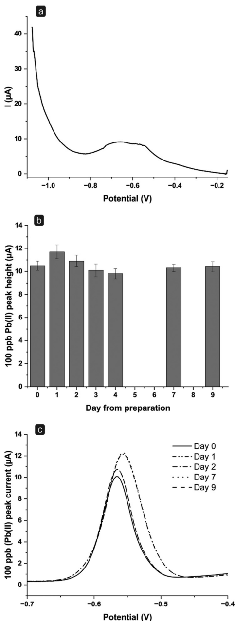
Fig. 6 (a) SWASV signal of a 0.1 M HCl solution containing 100 ppb \text{Pb(II)} on Day 3 using an external \text{Ag}/\text{AgCl} reference electrode. (b) Peak heights and (c) voltammograms obtained for 100 ppb \text{Pb(II)} using 0.1 M acetate buffer (pH 4.75) as medium to study the stability of the flow system during consecutive days; the bars represent average peak currents resulting from SWASV ( n = 6 per day, total number of measurements: 54); the potentials are referred to the external \text{Ag}/\text{AgCl} reference electrode.
