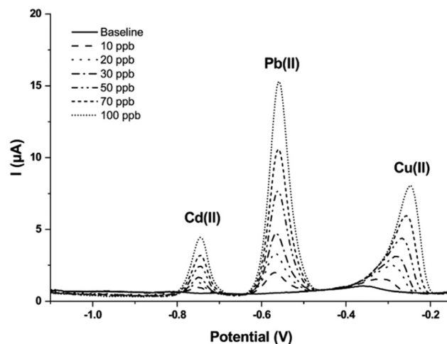
Fig. 7 SWASV scans obtained for \text{Cd(II)} , \text{Pb(II)} , and \text{Cu(II)} in the range 0–100 ppb under optimized conditions; the measurements were performed using 0.1 M acetate buffer (pH 4.75) as medium.
