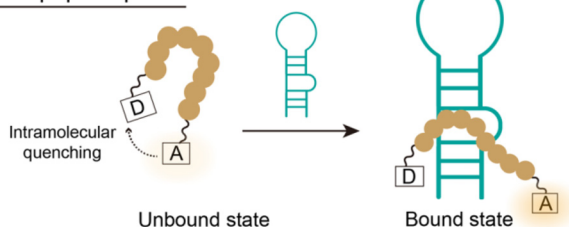
Fig. 1 Schematic illustration of the Tat peptide-based fluorogenic probe based on forced intercalation of the TO unit integrated into the middle of the peptide sequence as if it were a substitute for the amino acids that make up the Tat peptide. A traditional FRET-based probe was also shown as a comparison.
