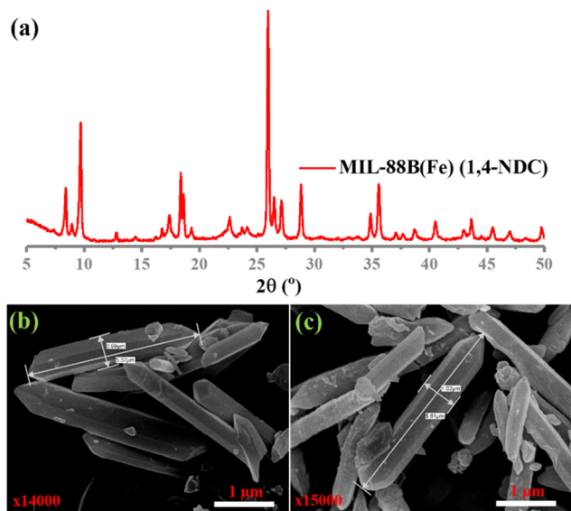
Fig. 1 (a) The PXRD pattern shows the as-synthesized MIL-88B(Fe) (1, 4-NDC) MOF. The FE-SEM images show (b) the as-synthesized MOF and (c) the MOF after incubation in an acidic buffer for 24 hours at pH 3.6.
