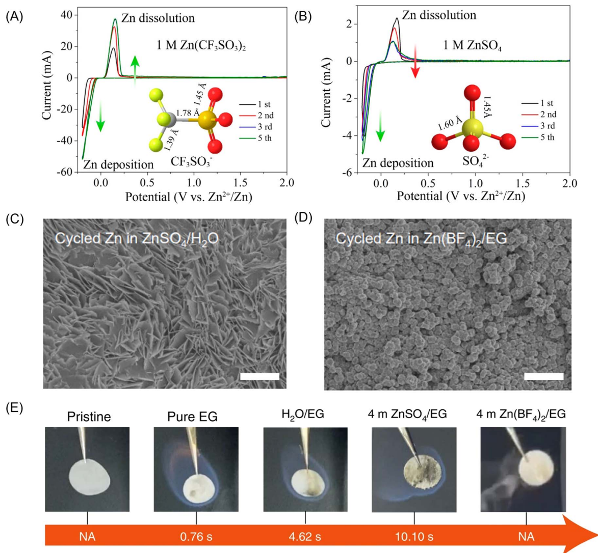
Fig. 6 Cyclic voltammetry of the Zn electrode in aqueous electrolyte of (A) 1 M \text{Zn}(\text{CF}_3\text{SO}_3)_2 and (B) 1 M \text{ZnSO}_4 at the scan rate of 0.5 \text{ mV s}^{-1} between -0.2 and 2.0 \text{ V} . Reproduced with permission. 102 Copyright 2016, American Chemical Society. Top-view SEM images of the cycled Zn after 20 cycles in (C) the reference aqueous \text{ZnSO}_4 electrolyte and (D) the 4 m \text{Zn}(\text{BF}_4)_2/\text{EG} electrolyte. (E) Ignition tests of a pristine glass fibre separator, one saturated with pure EG, a \text{H}_2\text{O}/\text{EG} solution, a 4 m \text{ZnSO}_4/\text{EG} solution and a 4 m \text{Zn}(\text{BF}_4)_2/\text{EG} solution. NA (not applicable) indicates non-flammability. Reproduced with permission. 101 Copyright 2021, Springer Nature.
