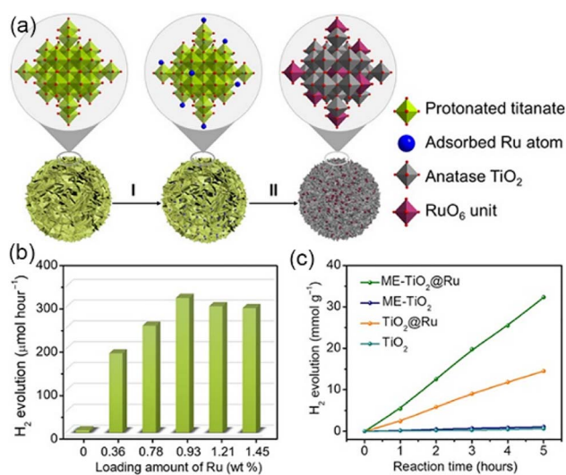
Fig. 4 (a) Illustration of the synthetic route to Ru SAs in TiO 2 . (b) Photocatalytic H 2 generation rates of ME-TiO 2 @Ru with different Ru loading amounts. (c) Time-dependent hydrogen evolution activities. Copyright 2020, the author, and American Association for the Advancement of Science.
