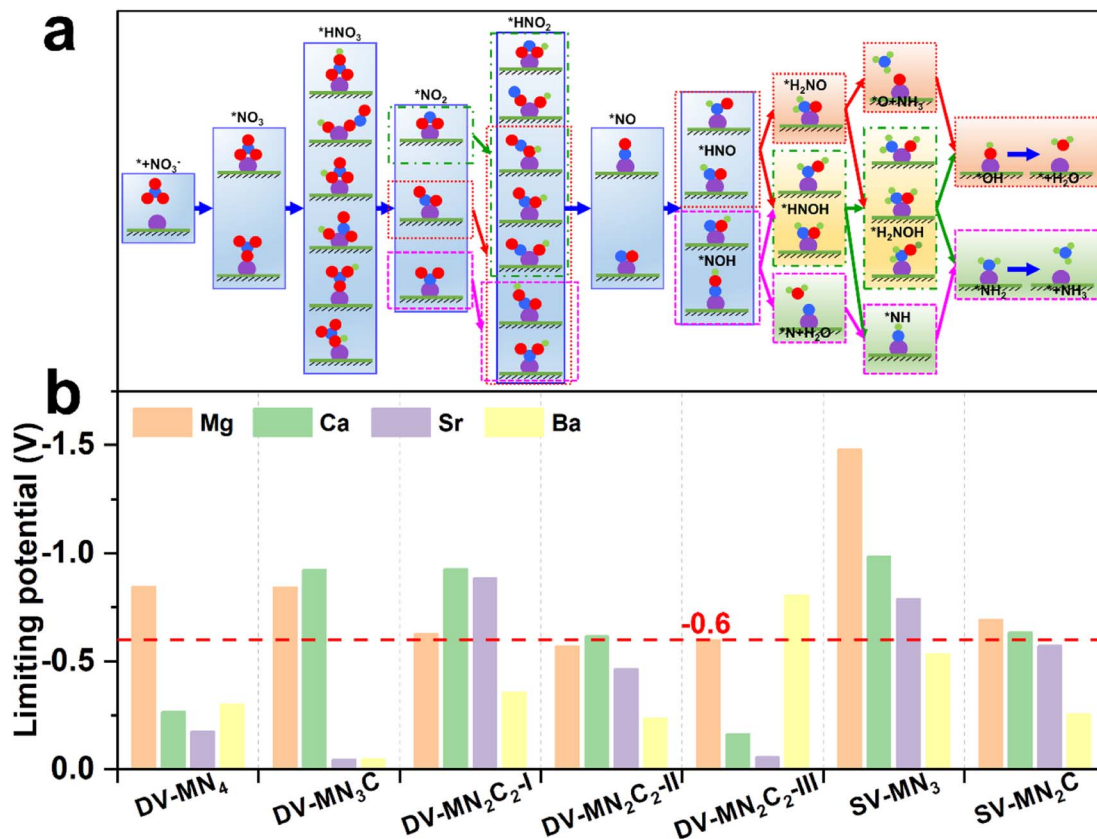
Fig. 4 (a) Schematic diagram of possible e\text{NO}_3\text{RR} pathways. (b) Summary of the limiting potential of the AE-SACs for e\text{NO}_3\text{RR} through the minimum energy pathway.
