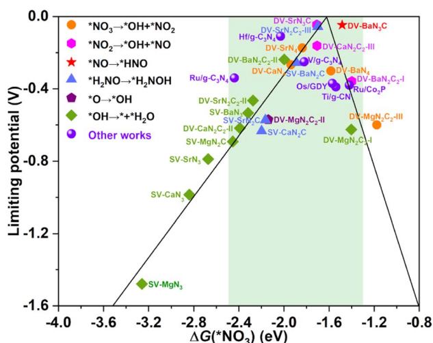
Fig. 5 The e\text{NO}_3\text{RR} volcano diagram of the considered AE-SACs with the descriptor of \Delta G(*\text{NO}_3) . The purple spheres denote other works for comparison 45–50 . The green background encloses those AE-SACs with acceptable limiting potentials.
