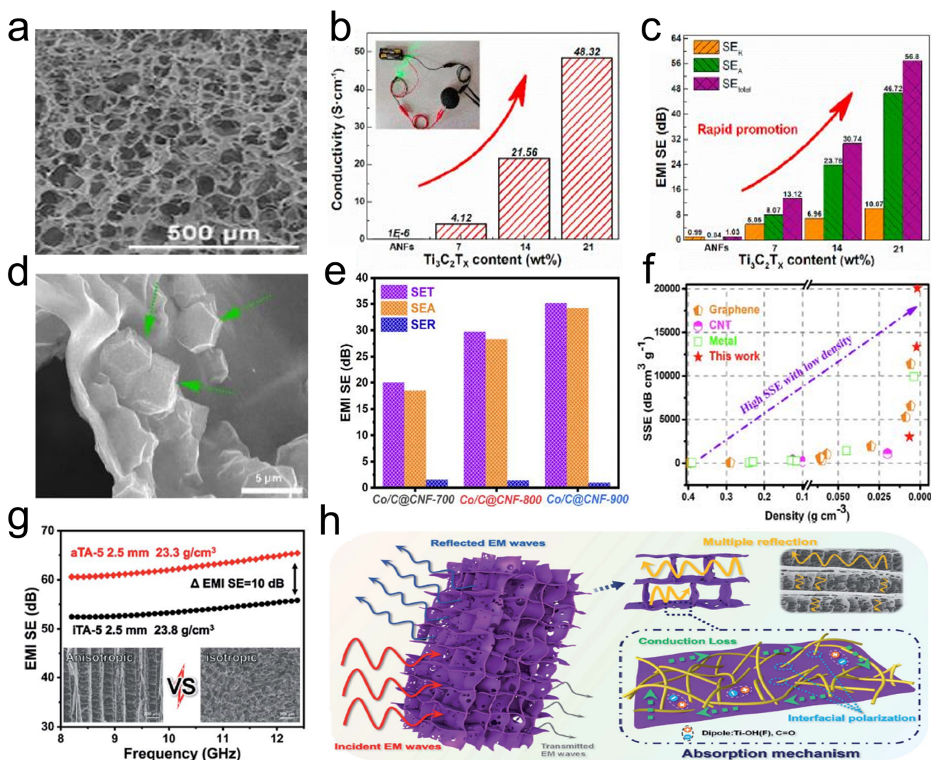
Fig. 19 3D fibrous hybrid aerogels for EMI. (a) SEM image, (b) histogram of electrical conductivity, and (c) comparison of microwave reflection (SE r ) and microwave absorption (SE a ) of a Ti 3 C 2 T x /ANF hybrid aerogel. Reproduced with permission. 58 Copyright 2017, Elsevier. (d) SEM image of the Co/C@cellulose nanofiber aerogel. (e) Average SET, SEA, and SER values in the X-band of Co/C@cellulose nanofiber aerogels with various temperatures. (f) Comparison of the shielding performance of any aerogels/foams/sponges ever reported. Reproduced with permission. 76 Copyright 2020, Elsevier. (g) A comparison of the anisotropic and isotropic Ti 3 C 2 T x /ANF aerogel. (h) EMI mechanism of the anisotropic Ti 3 C 2 T x /ANF aerogel. Reproduced with permission. 150 Copyright 2022, Royal Society Chemistry.
